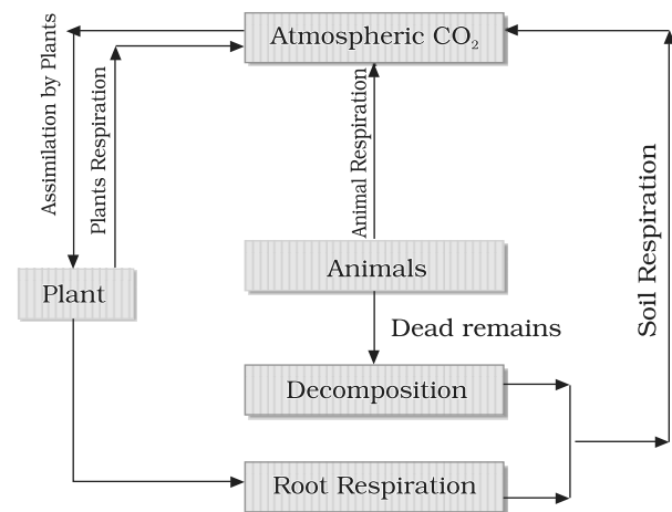
Figure 15.2 : Carbon Cycle
