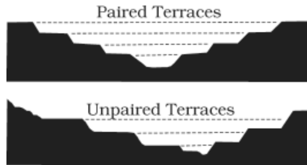
Figure 7.3 : Paired and unpaired river terraces
