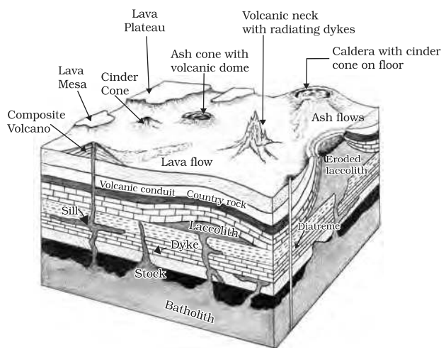
Figure 3.5 : Volcanic Landforms
